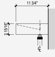
SIDE ELEVATION
