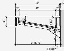
CROSS SECTION
