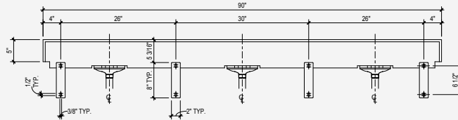
REAR ELEVATION
