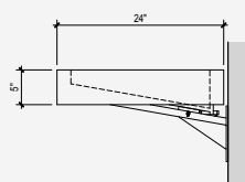
SIDE ELEVATION
