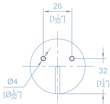
Fixing Locations
