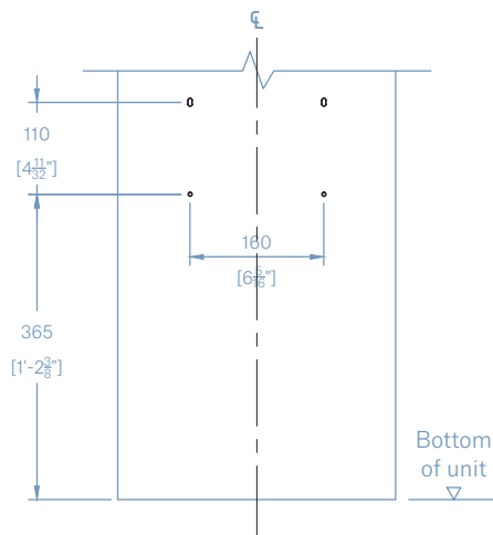
Fixing Positions
