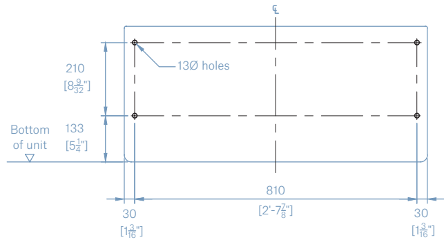
Fixing positions
