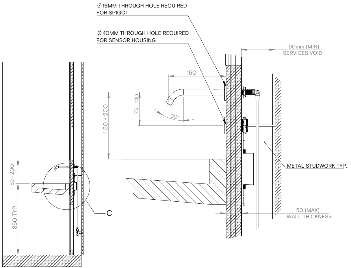
DETAIL C SCALE 1 : 5
